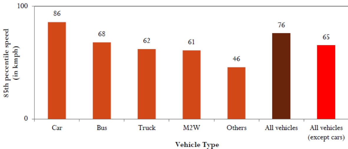
FIGURE 15: SPEED STUDY CONDUCTED BY JPRI ON A STATE HIGHWAY IN KARNATAKA
